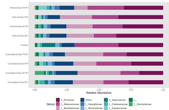
Figure 2.2. Relative Abundance of top 10 fungus from microbiomes of conjunctival swabs of infected and contralateral eye of Fusarium solani and Aspergillus flavus keratitis patients as well as review cases. Control groups is from cataract patients.
