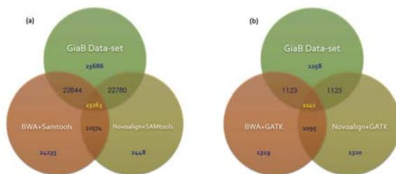
TP of GiaB data set's SNVs (a) and InDels (b) with pipelines.
