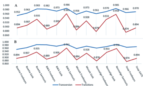
Figure 2 (A) Pipeline results for Transitions and Transversions of SNVs using (A) GiaB data and (B) simulated data
